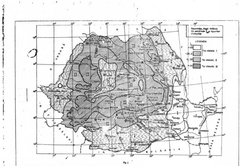
Fig. 7. Tipuri climatice (conform STAS-1709-1-90)
