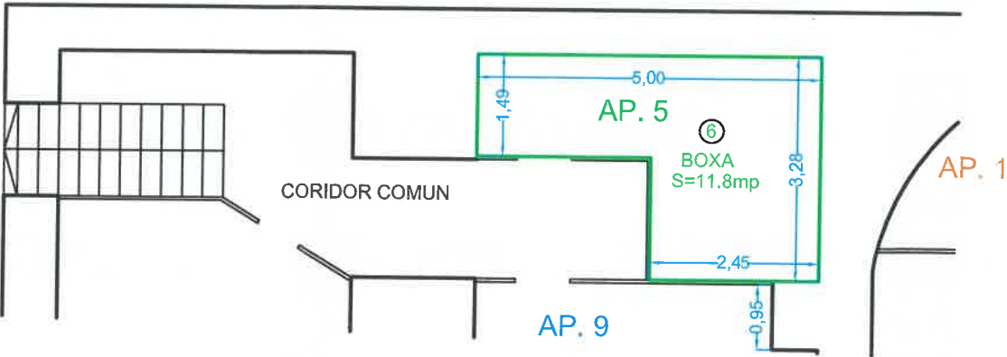
PLAN SUBSOL Scara 1:100
