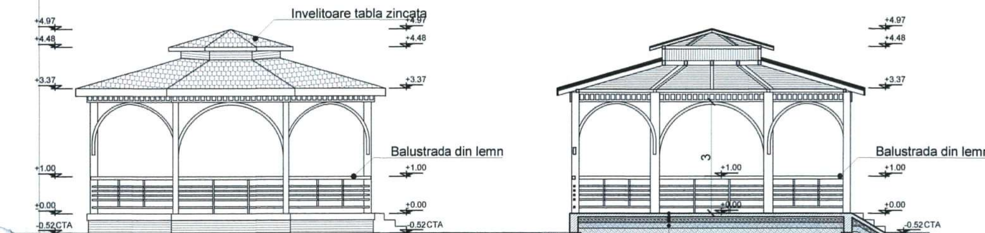
FATADA LATERALA sc. 1:100
